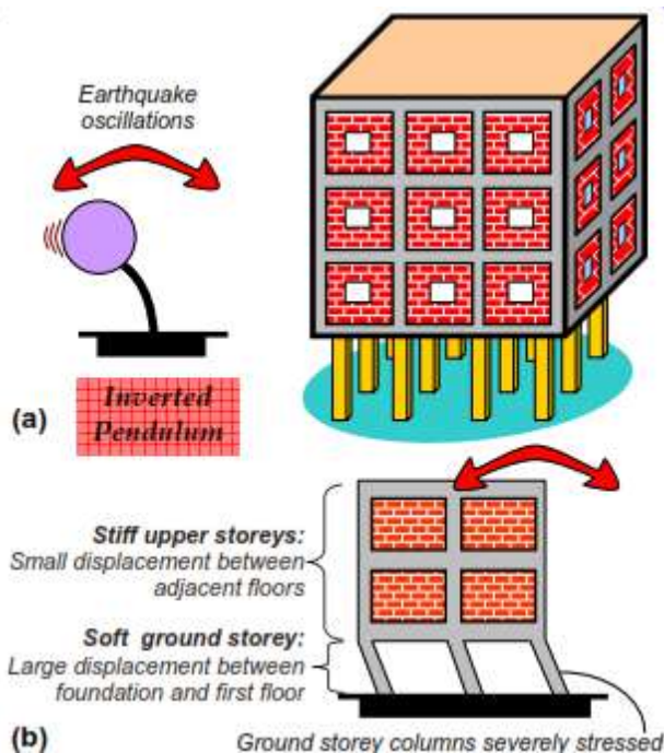
Fig- Upper storeys of open ground storey building move together as a single block – such buildings are like inverted pendulums
