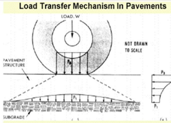
Figure 4 : Load transfer in rigid pavement
