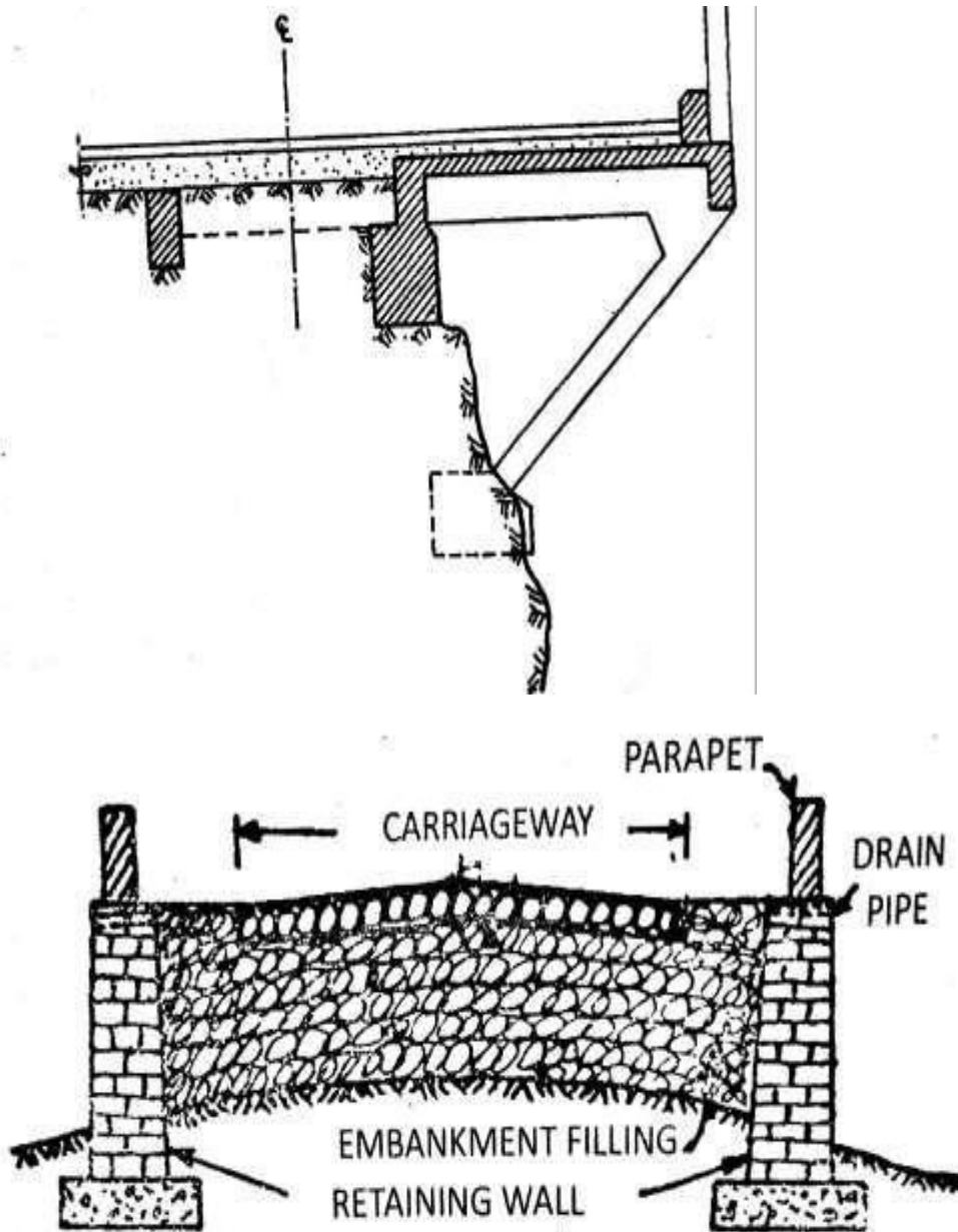
Fig: Fully In Embankment
