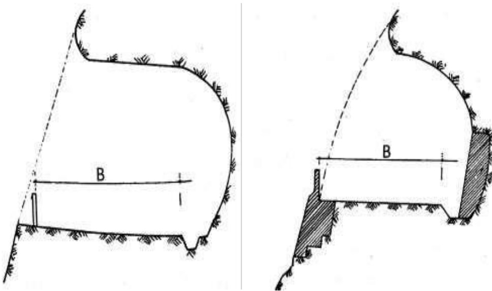
Fig: With Accommodating Road-Way Only and With Retaining and Breast Walls
