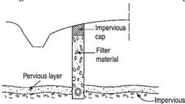
Fig. Subsurface drain to intercept drain water
