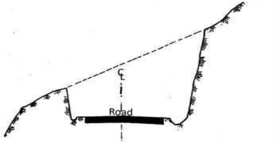
Typical Cross Sections of Box cutting
