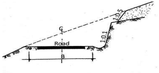
Typical Cross Sections of Bench type
