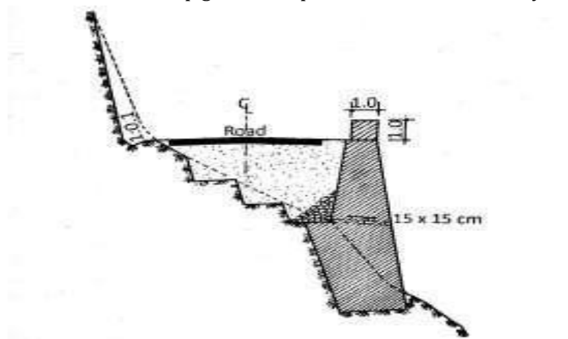
Typical Cross Sections of Embankment with retaining walls
